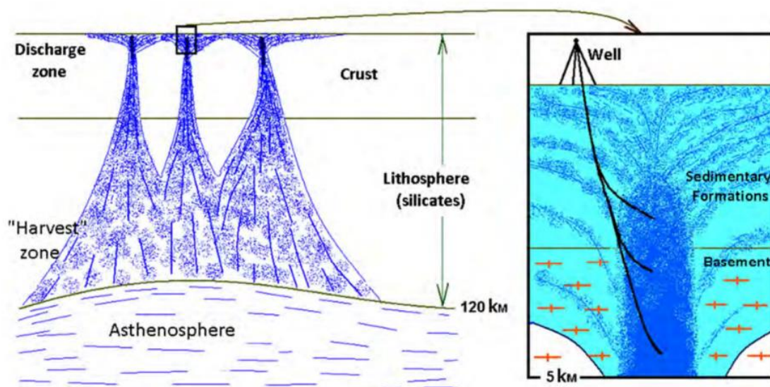
Hydrogen degassing in the lithosphere - Schematics
